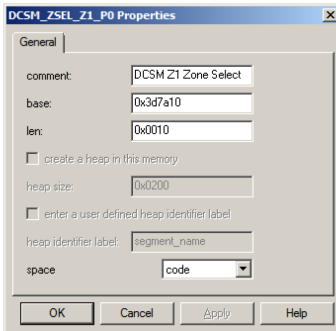
Figure 10. DSP/BIOS MEM Properties for DCSM_ZSEL_Z1_P0 Memory
